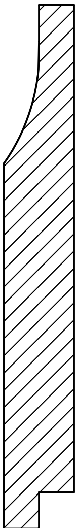
6" PATTERN 105 SIDING D & BETTER YELLOW PINE
