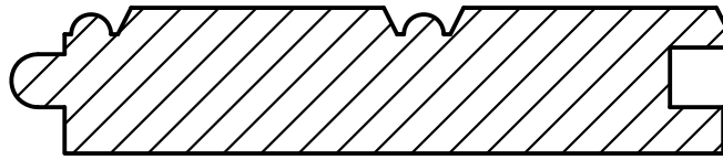
1x4 DOUBLE BEADED CEILING C & BETTER YELLOW PINE 3-1/8" FACE 3-3/8" OVERALL
