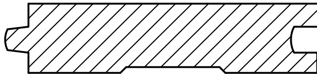
1x4 FLOORING C & BETTER YELLOW PINE PRESSURE TREATED CYP-KDAT 3-1/8" FACE 3-3/8" OVERALL
