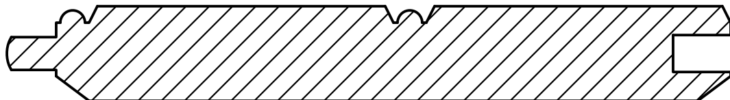
1x6 DOUBLE BEADED CEILING PRIMED F.J. WHITE PINE D & BTR WHITE PINE KNOTTY WHITE PINE 5-1/8" FACE 5-1/2" OVERALL
