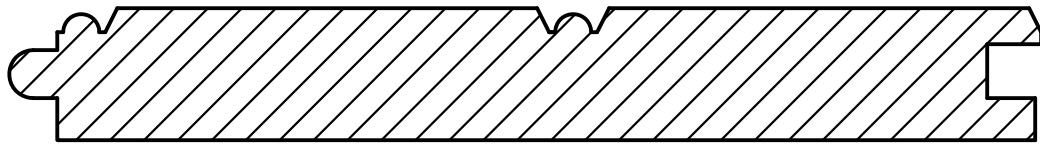
1x6 DOUBLE BEADED CEILING C & BETTER YELLOW PINE 5-1/8" FACE 5-3/8" OVERALL
