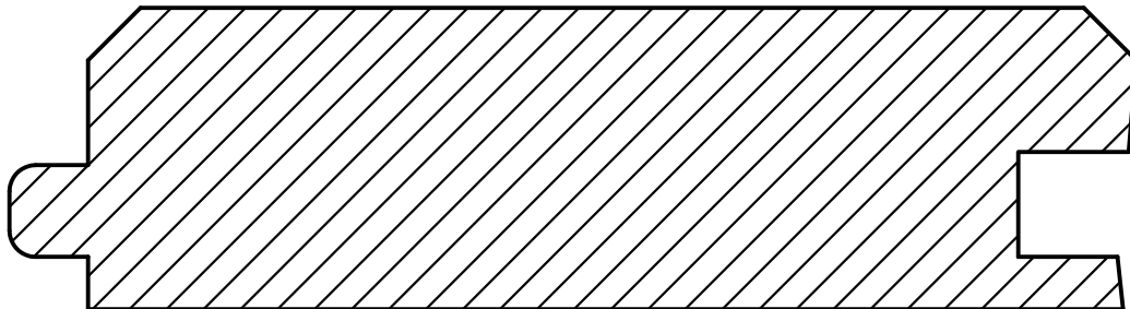
2x6 T&G V-JOINT #1 YELLOW PINE 5" FACE 5-3/8" OVERALL
