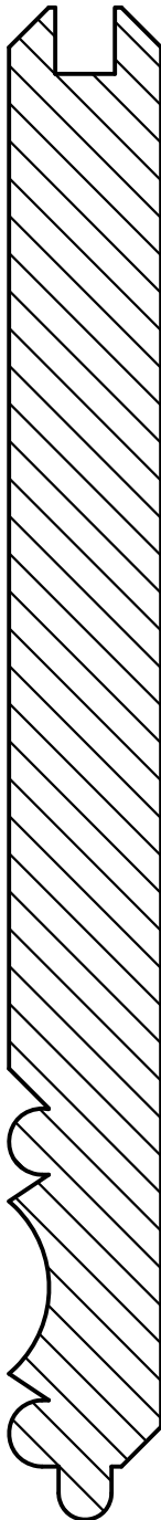
8" PICKWICK / T&G V-JOINT KNOTTY WHITE PINE - 8' & 10' LENGTHS ONLY 6-7/8" FACE 7-1/8" OVERALL
