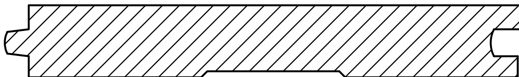
1x6 FLOORING C & BETTER YELLOW PINE 5-1/8" FACE 5-3/8" OVERALL
