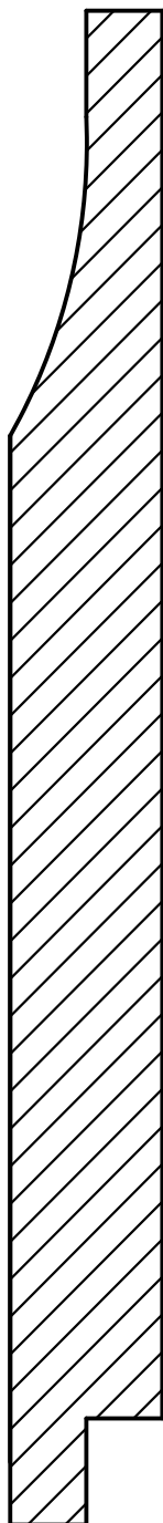
8" PATTERN 105 SIDING D & BETTER YELLOW PINE
