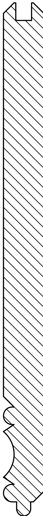
10" PICKWICK / T&G V-JOINT KNOTTY WHITE PINE - 8' & 10' LENGTHS ONLY 8-7/8" FACE 9-1/8" OVERALL
