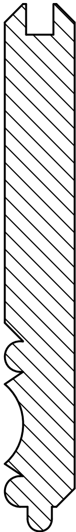
6" PICKWICK / T&G V-JOINT KNOTTY WHITE PINE - 8' & 10' LENGTHS ONLY 5-1/8" FACE 5-3/8" OVERALL
